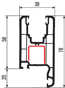
PRS602B Kanat Profili Sash Profile
