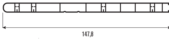
PRPJ63 Panjur Kutu Alt Kapak Profili Shutter Box Bottom Cover Profile
