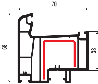
PRP711-T Geniş Kanat Profili Wide Sash Profile
