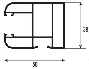
PRPJ55 Panjur Kenar Yan Ray Dikme Rail Shutter Edge Side Pillar
