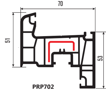
PRP702 Kanat Profili Sash Profile DS-12
