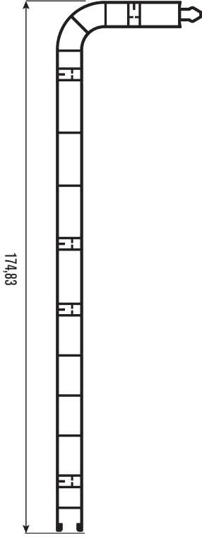
PRPJ62 Panjur Kutu Radyuslu Yan Kapak Profili Shutter Box Side Cover Profile radius
