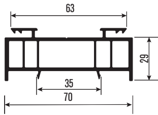
PRP737 Kasa Yükseltme Profili Frame Joint Profile
