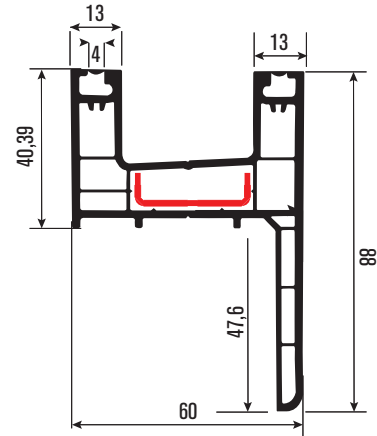
PRS608B Pervazlı Kasa Profili Casing Frame Profile
