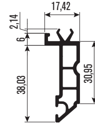
PRTS36 Dekoratif Pervaz Profili Decorative Casing Profile
