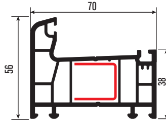
PRP706 Dar Kasa Profili Narrow Frame Profile DS-4
