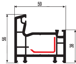
PRLT01 Kasa Profili Frame Profile DS-13 DS-20
