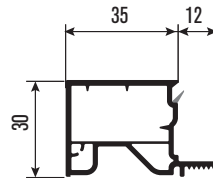
PRP783 35 mm Parapet 35mm Parapet
