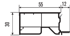
PRP784 55 mm Parapet 55mm Parapet
