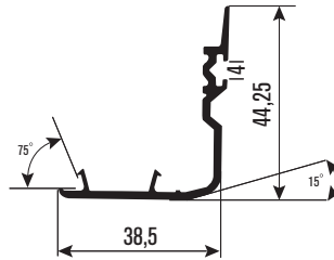
PRS638 Kanat Adaptörü Sliding Sash Adaptor
