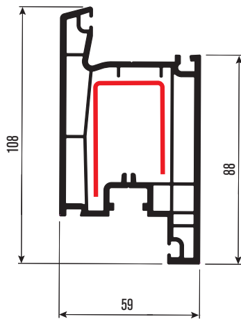
PR6004 Kilitli Kapı Profili-2 Door Sash Profile-2 DS-28 DS-14
