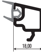
PR6017 20mm Çıta 20mm Glazing Bead
