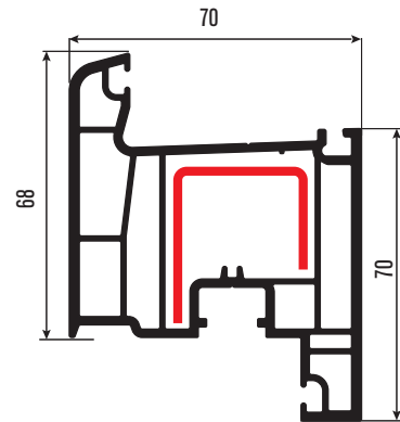
PRP704 Kapı Profili Door Profile DS-9
