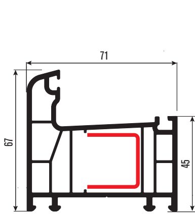
PRDR01 Kasa Profili Frame Profile DS-2 DS-3
