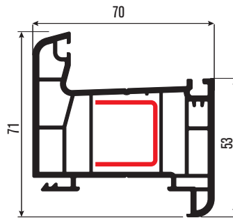
PRP776 Kısa Pervazlı Kasa Short Casing Frame Profile DS-2
