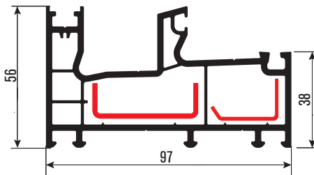
PRSY46 Fix Kasa Profili Fix Frame Profile
