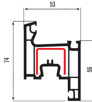
PRFS02 Kanat Profili Sash Profile DS-12
