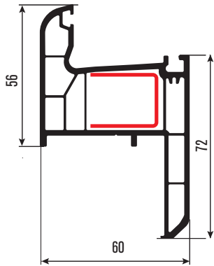
PRVN08 Pervazlı Kasa Profili Casing Frame Profile DS-3
