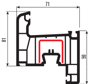
PR7102 Kanat Profili Sash Profile DS-2
