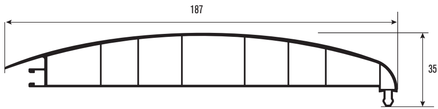
PRPJ80 Kutu Oval Elliptical Box
