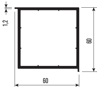
PR6033 60x60 Kutu Profili 60x60 Box Profile
