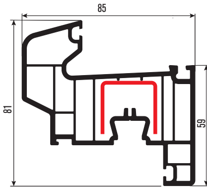
PR7107 Damlalıklı Kanat Profili Drained Sash Profile DS-2
