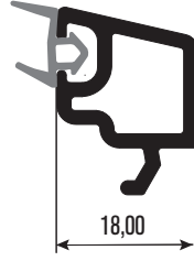
PR6017 20mm Çıta 20mm Glazing Bead
