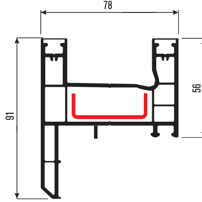
PRSY08 Pervazlı Kasa Profili Casing Frame Profile DS-05
