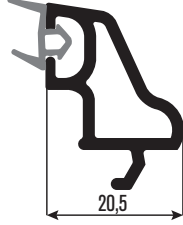
PR7121 30mm Çıta 30mm Glazing Bead
