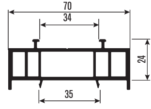
PR7137 Kasa Yükseltme Frame Joint Profile
