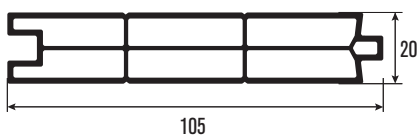
PRTS22 Lambri Panel
