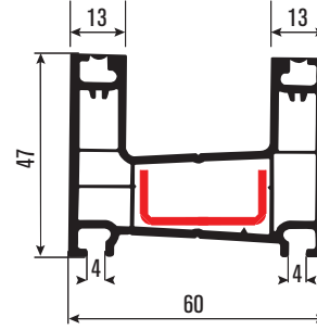
PRS601B Kasa Profili Frame Profile
