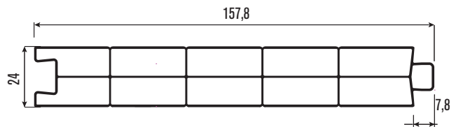
PRTS23 Lambri 24 mm Panel 24 mm
