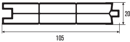
PRTS22 Lambri Panel
