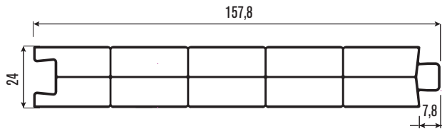
PRTS23 Lambri 24 mm Panel 24 mm
