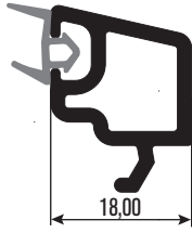
PR6016 20mm Çıta 20mm Glazing Bead
