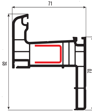
PR7108 Pervazlı Kasa Profili Casing Frame Profile DS-3
