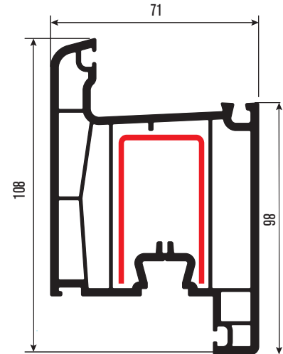
PR7104 Kilitli Kapı Profili Door Sash Profile DS-8 DS-14
