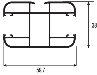
PRPJ56 Panjur Orta Ray Dikme Profil Shutter Central Rail Pillar Profile
