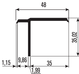
PRTS31 Asimetrik T T Covering
