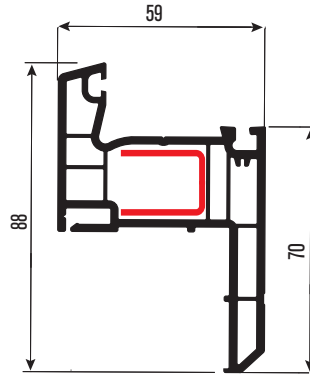
PR6008 Pervazlı Kasa Profili Casing Frame Profile DS-4
