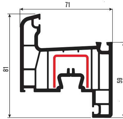
PR7102 Kanat Profili Sash Profile DS-2
