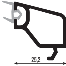
PR7119 24mm Çıta 24mm Glazing Bead
