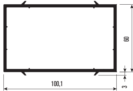
PR6034 60x100 Kutu Profili 60x100 Box Profile
