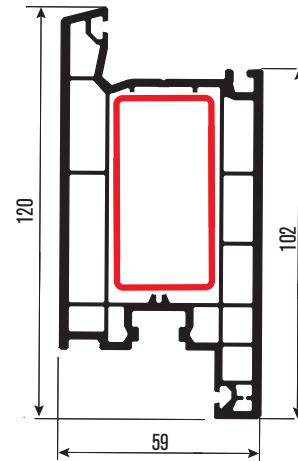
PR6012 Kilitli Kapı Profili-1 Door Sash Profile-1 DS-6 DS-15 DS-6
