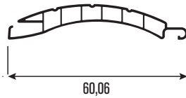
PRPJ58 Panjur 52'lik Lamel Profili Shutter 52 Lamella Profile
