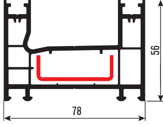
PRSY01 Kasa Profili Frame Profile DS-05
