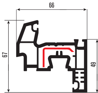
PR6007 Damlalıklı Kanat Formu Draned Sash Profile DS-13
