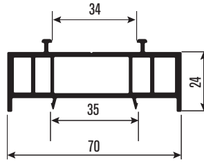
PR7137 Kasa Yükseltme Frame Joint Profile
