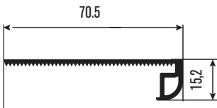
PRP787 Geçme 15 mm Pervaz Passing 15 mm Architrave
