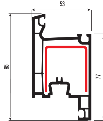
PRFS04 Kilitli Kapı Profili Door Sash Profile DS-10
