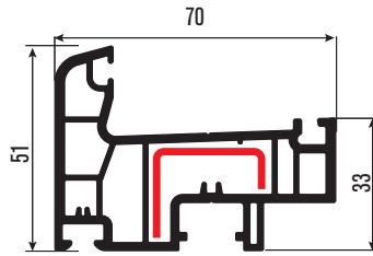
PRP710-T Dar Kanat Profili Narrow Sash Profile DS-12
