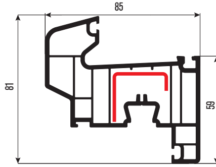
PR7107 Damlalıklı Profil Draned Sash Profile DS-12
