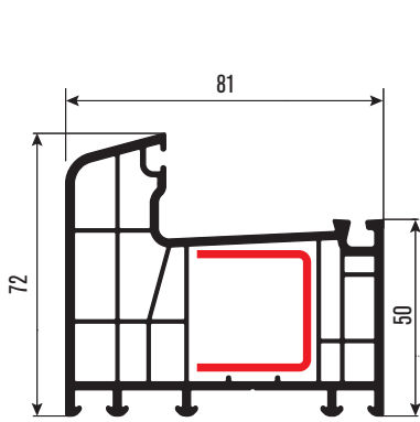
PRGR01 Kasa Profili Frame Profile DS-1
