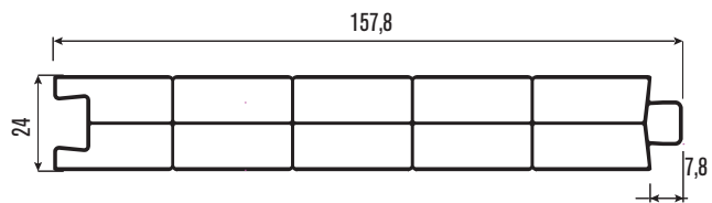
PRTS23 Lambri 24 mm Panel 24 mm
