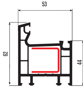
PRFS01 Kasa Profili Frame Profile DS-2
