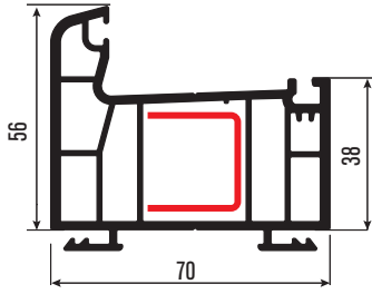
PRP701 Kasa Profili Frame Profile DS-2
