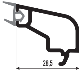
PR7117 20mm Çıta 20mm Glazing Bead
