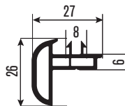
PRP738 Kanat Adaptörü Sash Adapter
