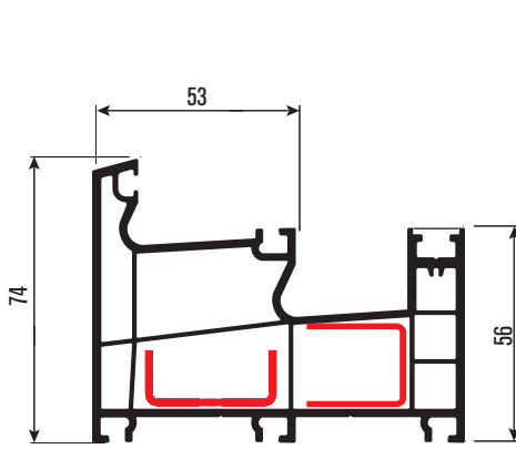
PRSY51 Dış Fix Kasa Profili Outside Fix Frame Profile
