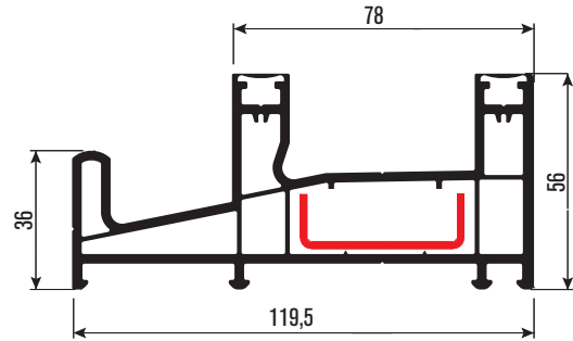
PRSY47 Sineklikli Kasa Profili Frame Fly Screen Profile DS-05
