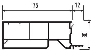
PRP785 75mm Parapet 75mm Parapet
