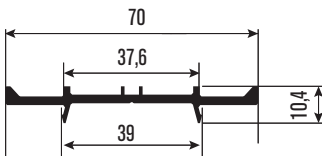
PRP786 Panjur Bağ Shutter Coupling
